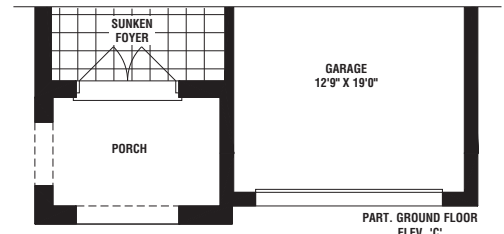
PART. GROUND FLOOR ELEV. 'C'
